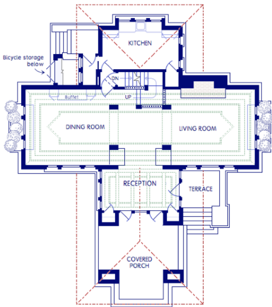
GEORGE BARTON HOUSE • BUFFALO NY • FRANK LLOYD WRIGHT • 1903–4 after Wasmuth Plate XXVI
